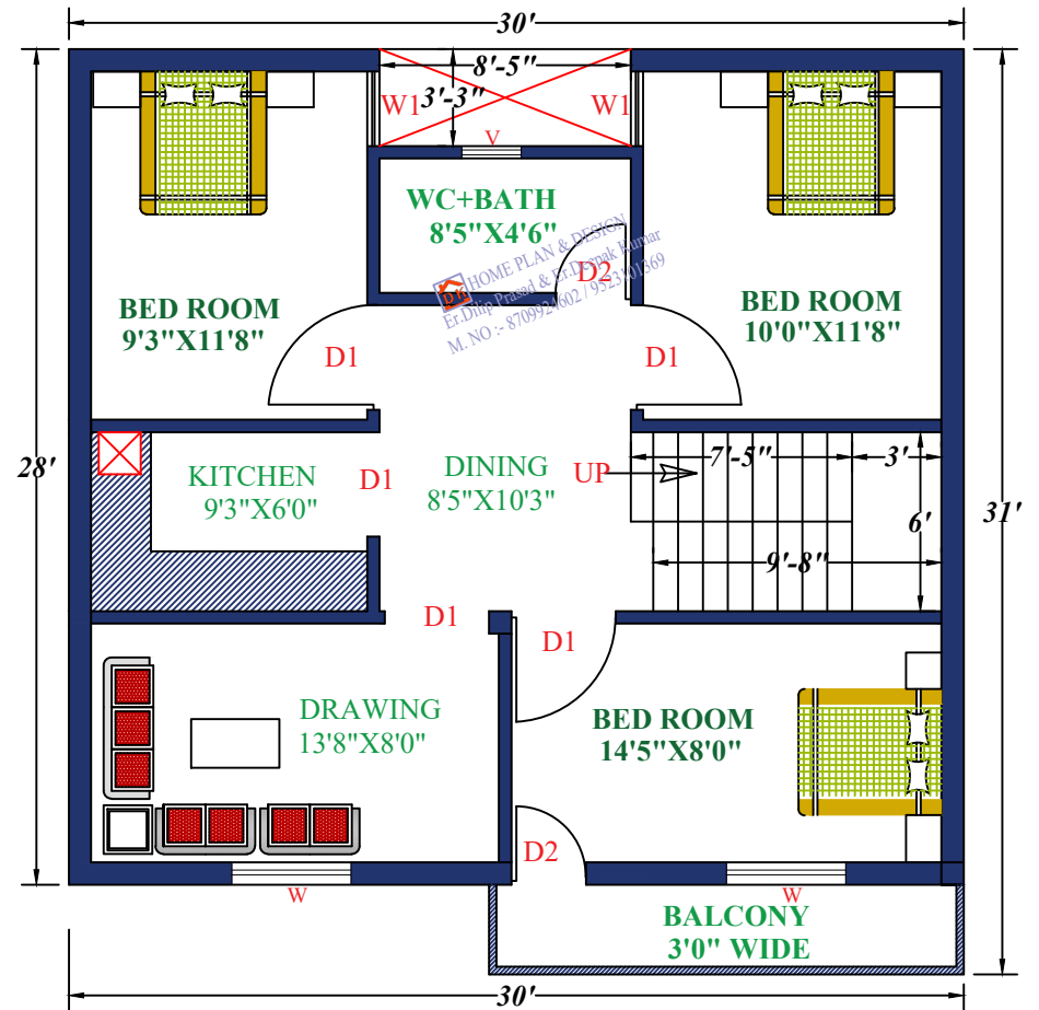
1ST FLOOR
