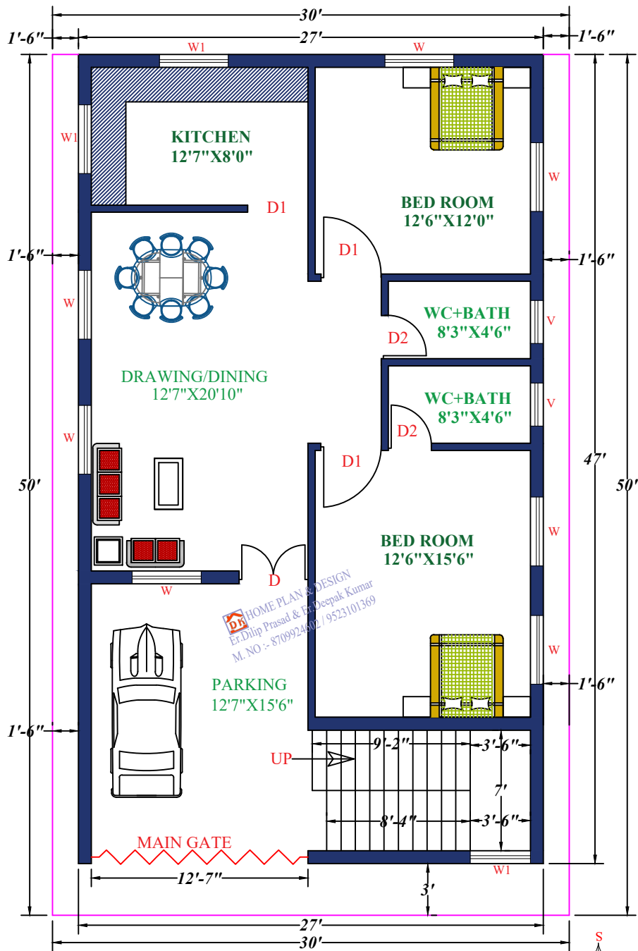
GROUND FLOOR
