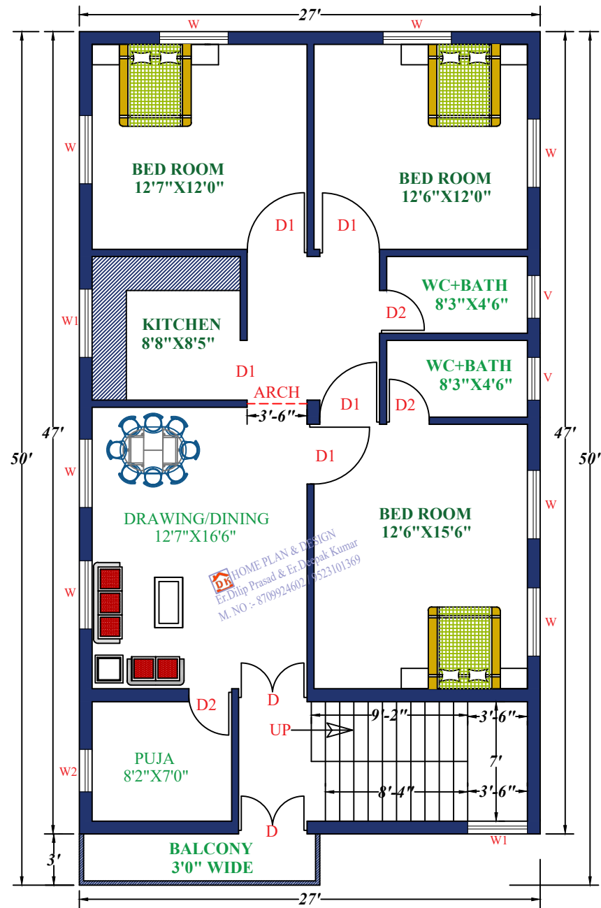
1ST FLOOR
