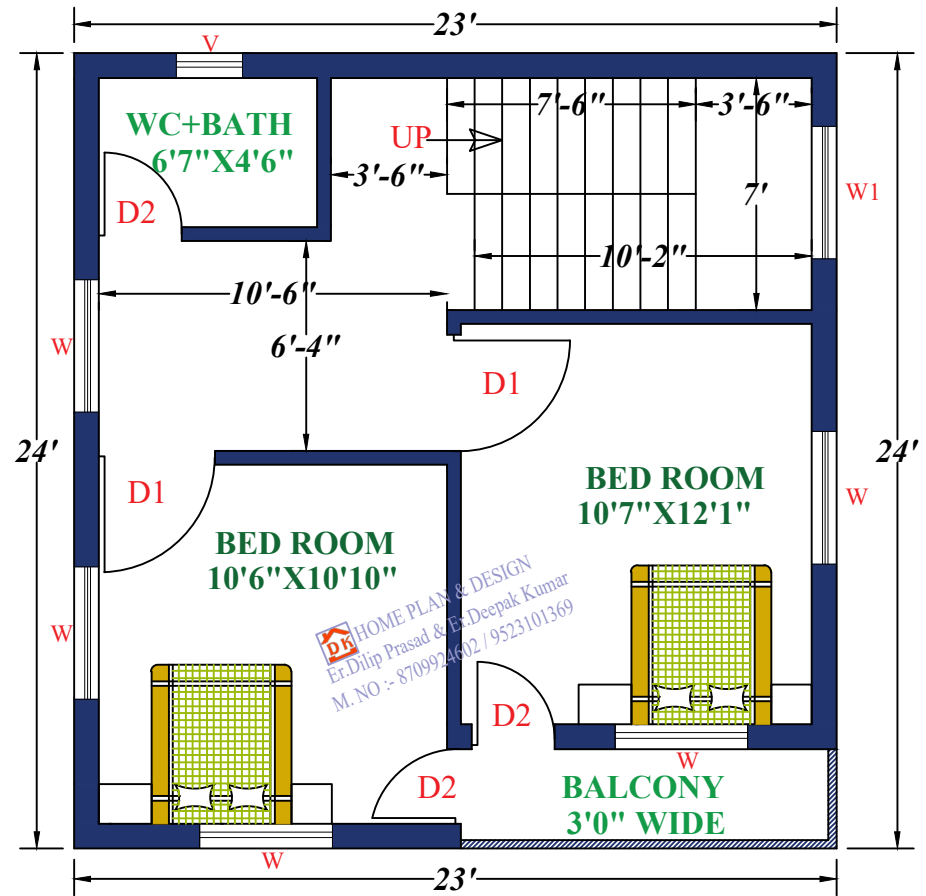
1ST FLOOR
