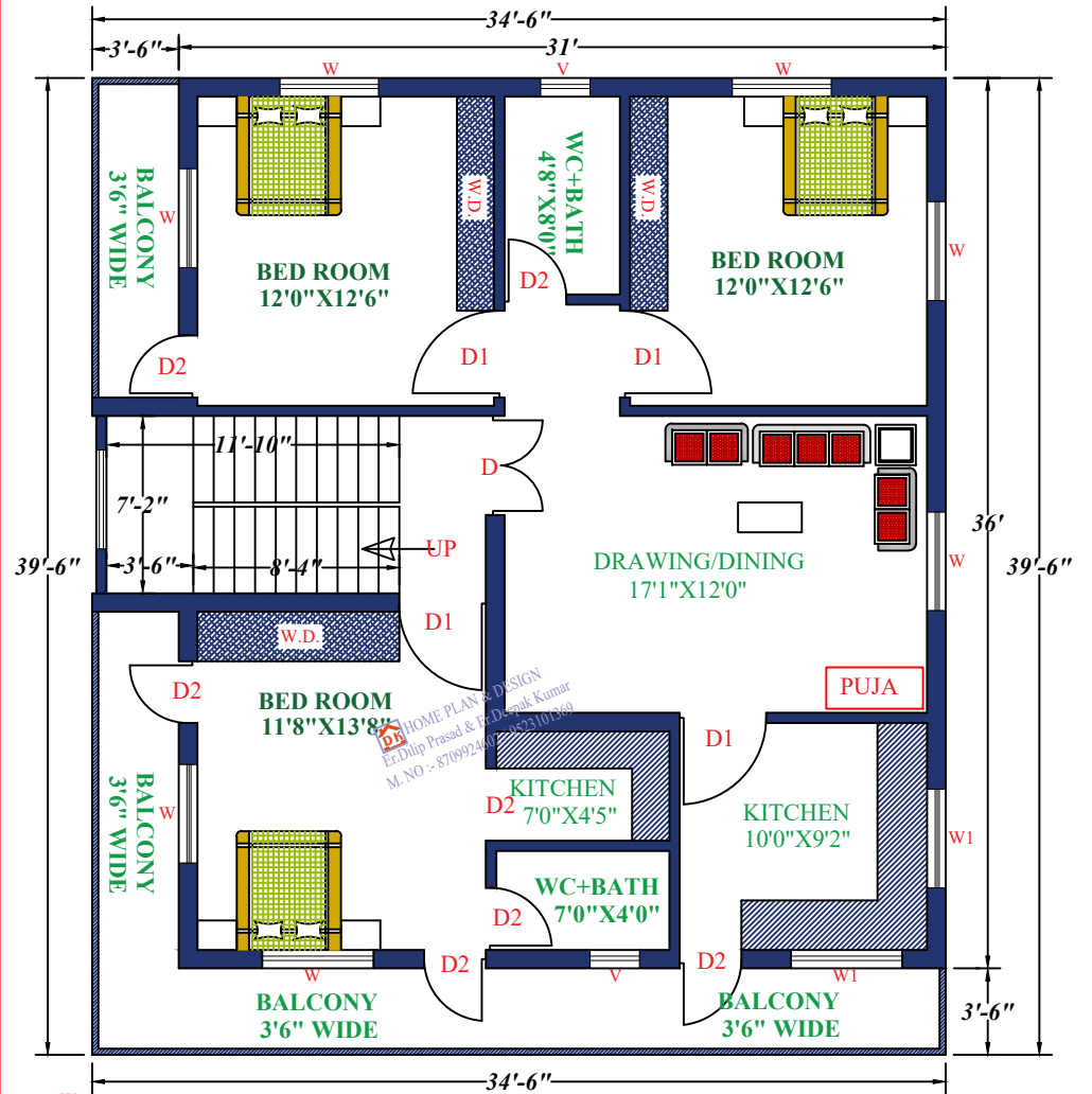
1ST FLOOR
